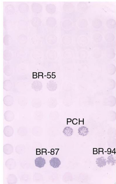
Figure 1. Nitrocellulose spot assay of duplicate bacteriophage clones expressing 44 different serologically-defined breast cancer antigens. Following incubation in a 1:200 dilution of serum from a colon cancer patient, the membrane was exposed to alkaline phosphatase-conjugated, Fc fragment-specific, goat anti-human IgG. A positive color reaction with 4-nitro blue tetrazolium chloride/5-bromo-4-chloro-3-indolyl-phosphate indicates seroreactivity with nucleosome assembly protein-1/NY-BR-55, NY-BR-87 and p53/BR-94, as well with the positive control antigen PINCH (PCH)/NY-CO-22.
